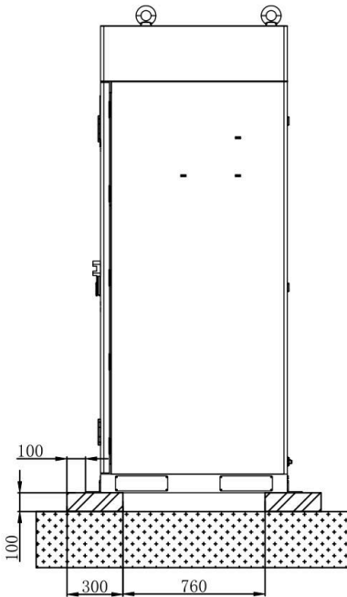
load-bearing surface
